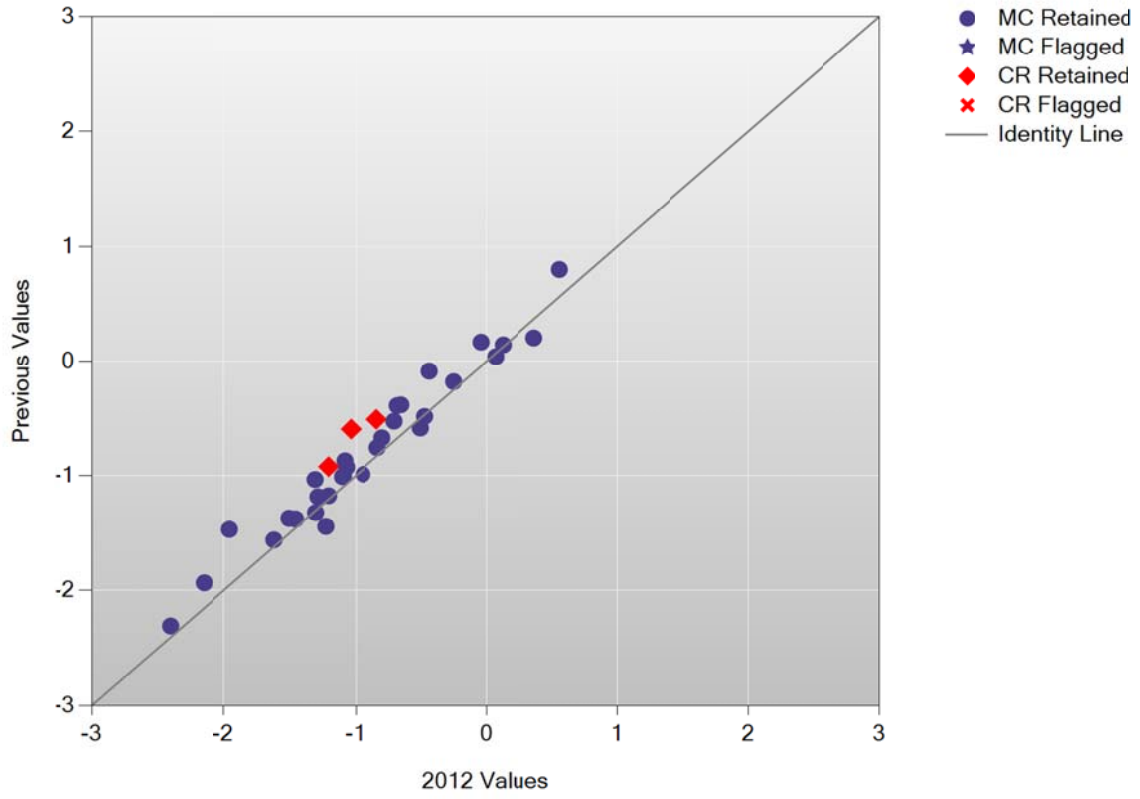
B/B Plot: English Language Arts Grade 8
